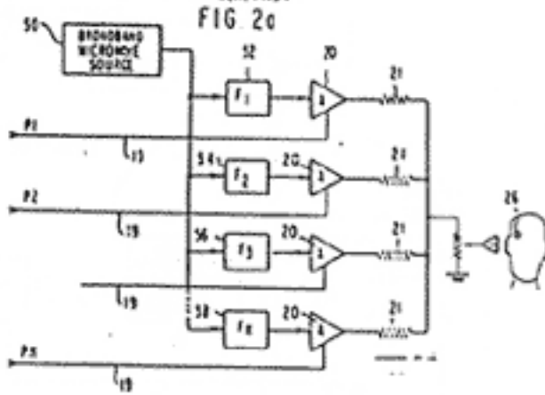
MICROWAVE RADIATOR GENERATOR
